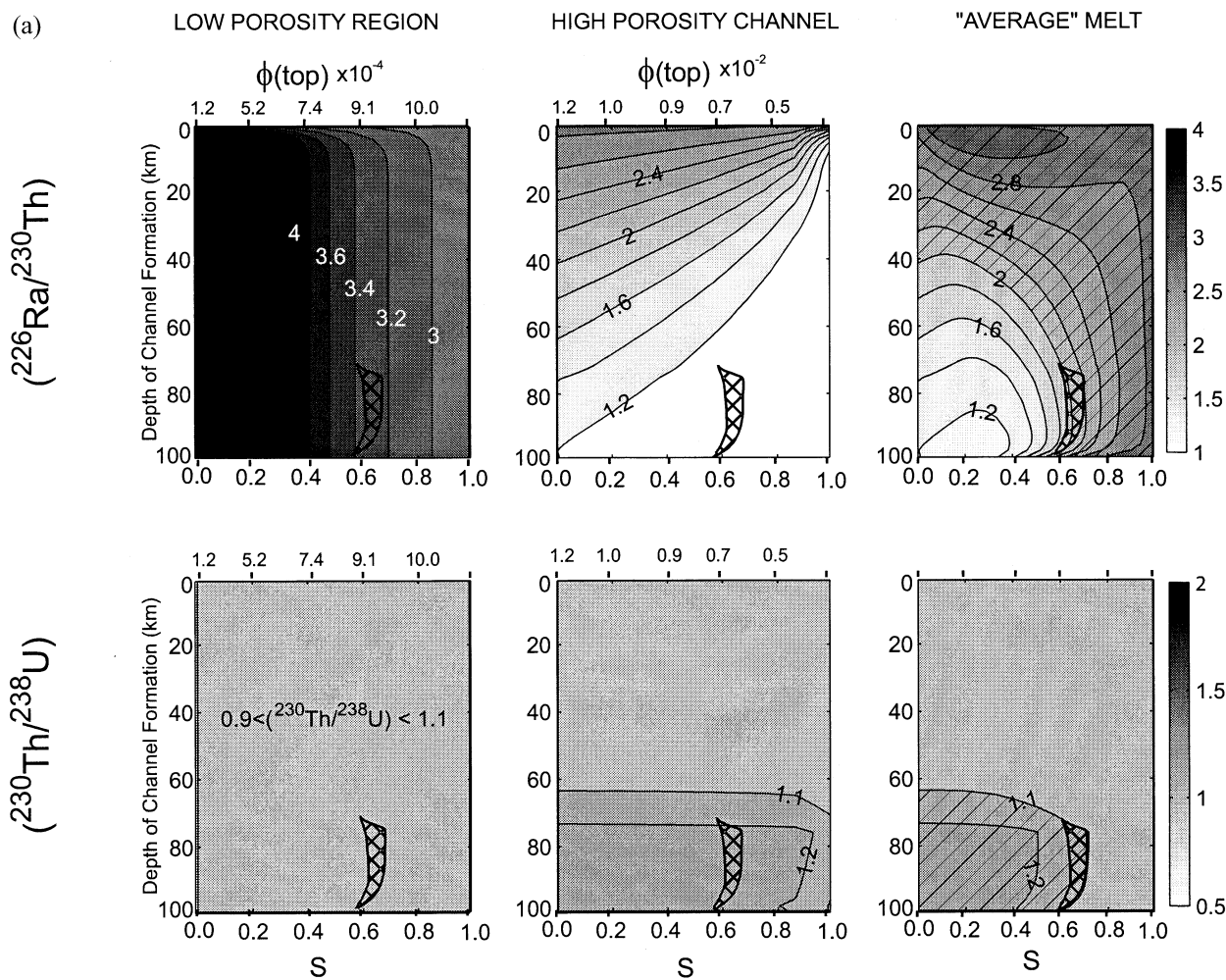
Fig. 4. Contours of calculated activity ratios at the top of the low-porosity region and the top of the high-porosity channels, and the average activity ratio of the melt as a function of the depth of channel formation and fraction of the total melt flux that remains in the low-porosity region S . In (a), K_{\text{cpx}} for U and Th are 3 \times 10^{-2} , and in (b) 0.5 \times 10^{-2} . For the average melt activity ratio, regions of the contour plot that are in the range of the average MORB data are marked with diagonal lines. The intersection of these regions for both ^{230}\text{Th} and ^{226}\text{Ra} activity ratios is marked by a "hatched" region which delineates the parameter range required to reproduce the average and end-member MORB data. In (b) there are no diagonal lines because the MORB data cannot be produced with the parameter range shown. In these calculations F = 0.15 , \chi = 0.01 , and V_0 = 1 cm/yr. See the text for further details.
